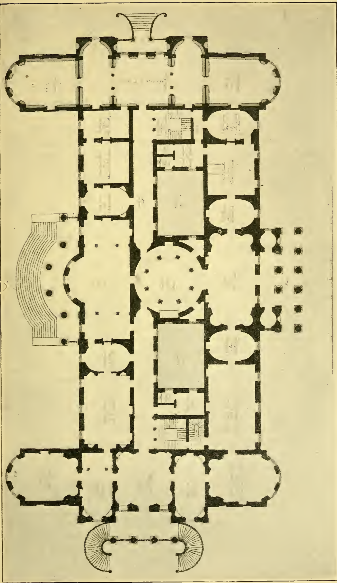
PLAN OF LUTON HOUSE.
